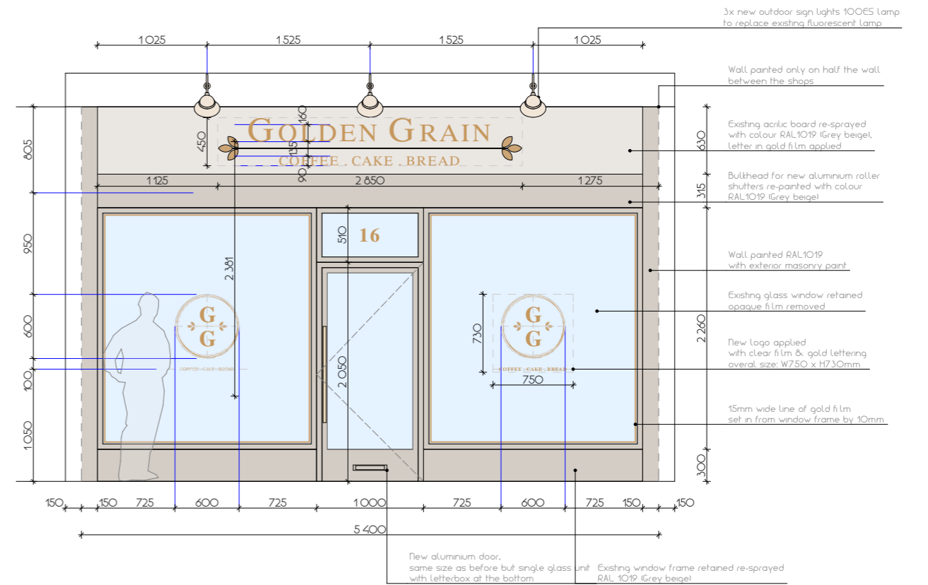
6 ELEVATION, PROPOSED SHOP FRONT SCALE: 1:50
