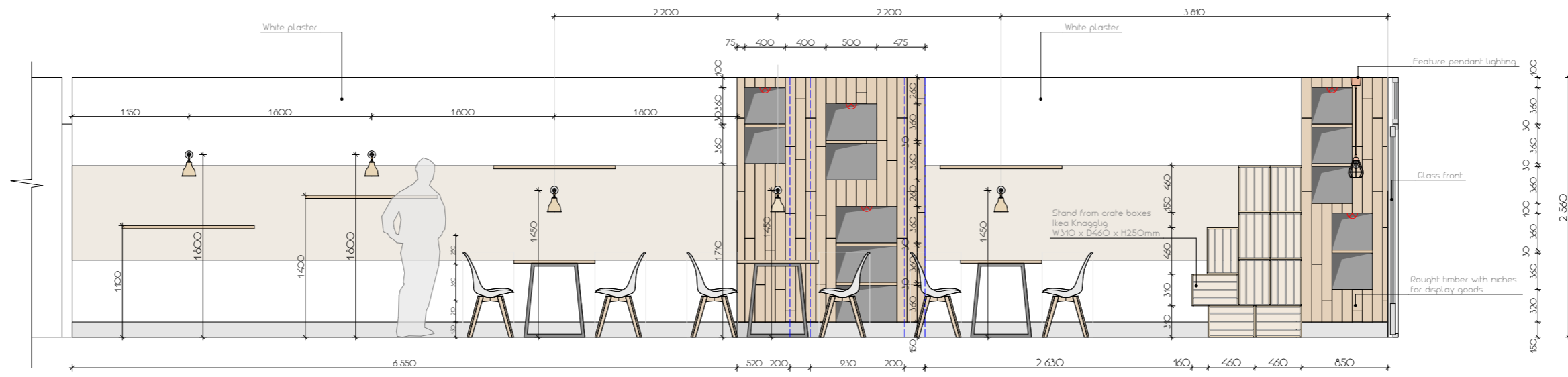
1 ELEVATION SEATING WALL A-2 SCALE: 1:50
