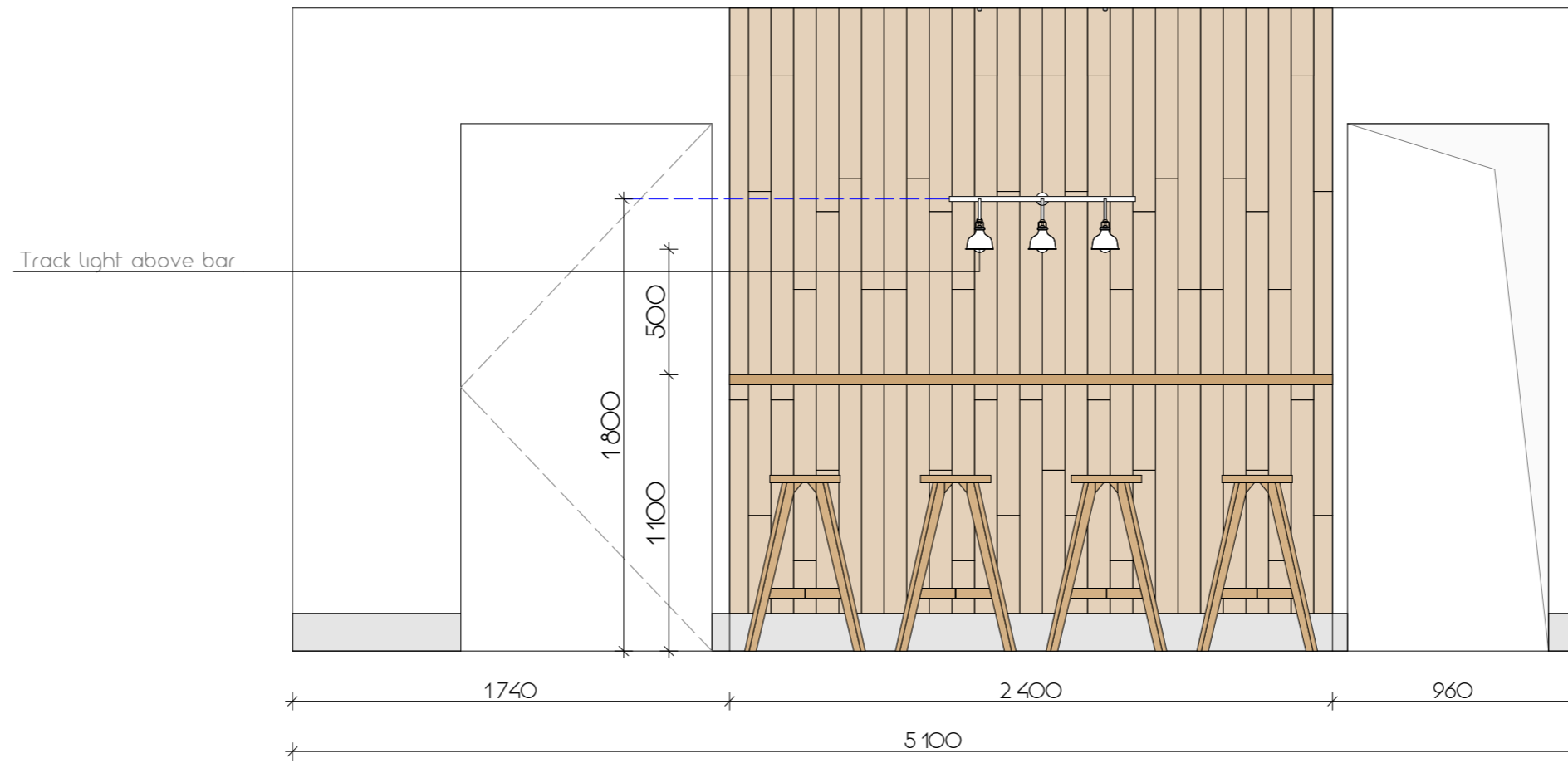
4 A-4 ELEVATION. OFFICE WALL SCALE: 1:25
